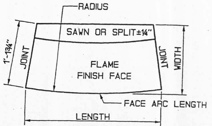
APPROVED ALTERNATE CIRCULAR CURB TYPE 5 2'-0" TO 8'-0" RADIUS
