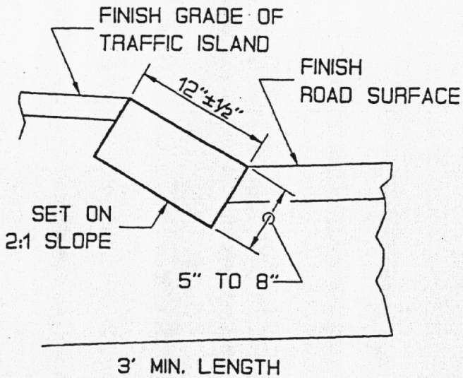
APPROVED ALTERNATE CIRCULAR CURB TYPE 5 2'-0" TO 8'-0" RADIUS
