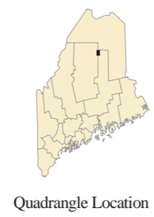
Quadrangle Location
