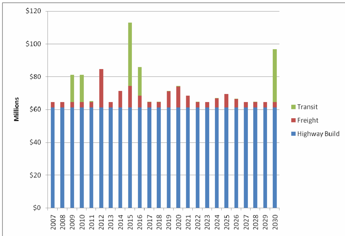
Figure 1 Construction Expenditures by Transportation System Component 2007-2030
