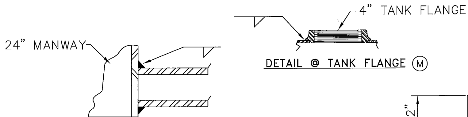
DETAIL @ MANWAY (A)
