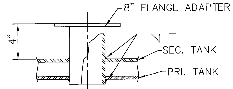
DETAIL @ PRI. EMER. VENT (B)
