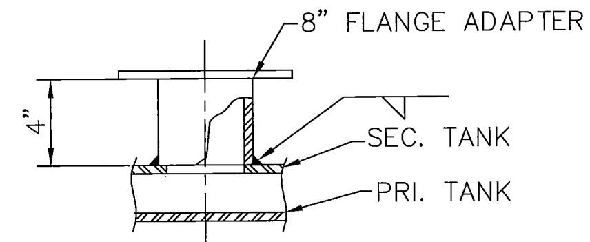
DETAIL @ SEC. EMER. VENT (C)
