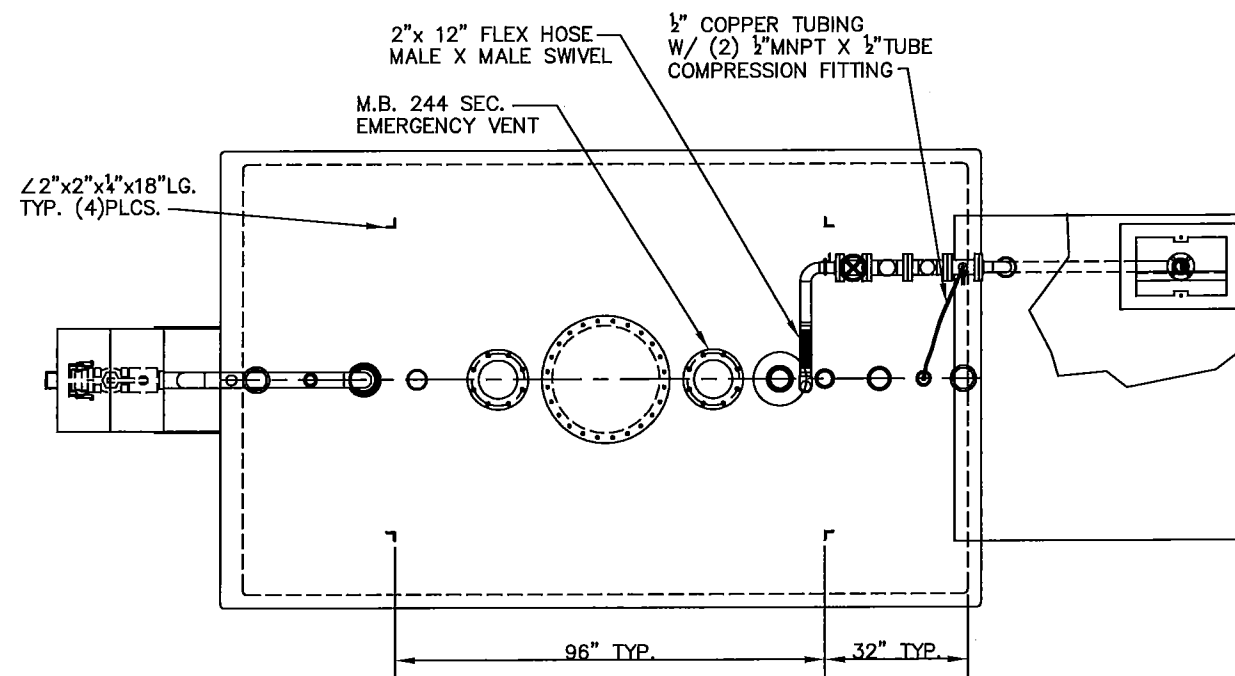
PLAN VIEW
