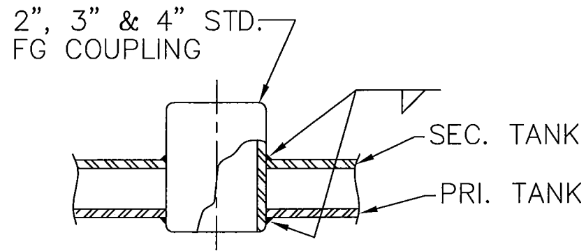
DETAIL @ COUPLINGS (G)(H)(J)(K)(L)
