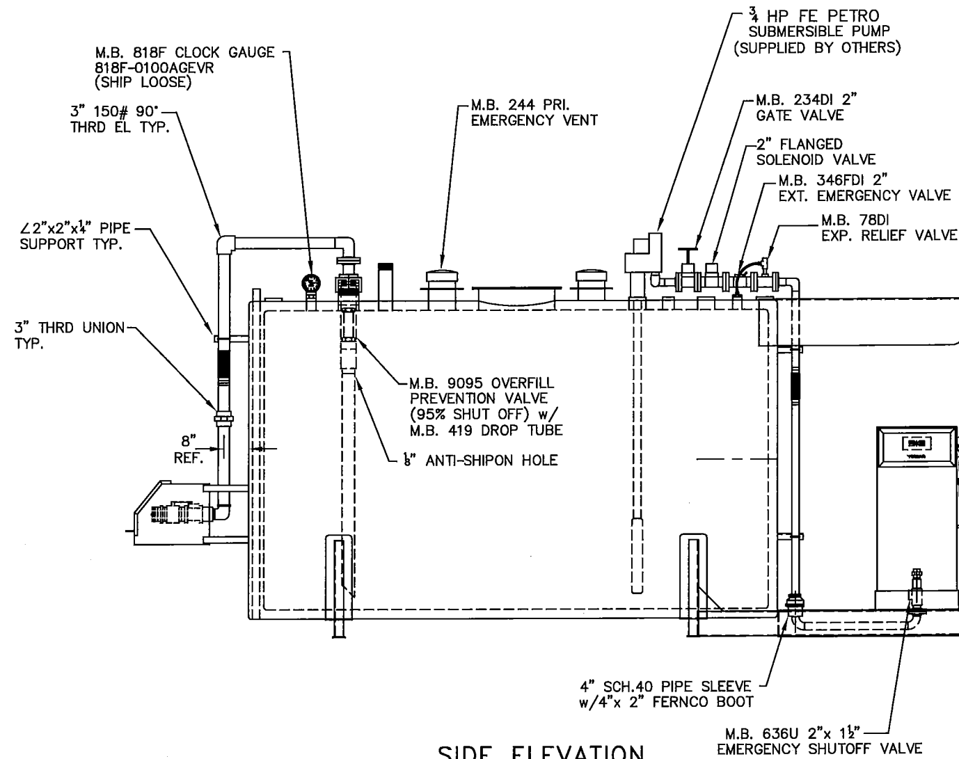
SIDE ELEVATION
