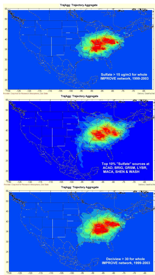
Figure 5-7. Comparison of probability fields for observed sulfate, "sulfate" source profiles for seven eastern sites and reconstructed deciviews
