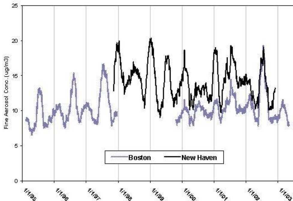
Figure 2-9. Moving 60-day average of fine aerosol mass concentrations based on long-term data from two northeastern cities
