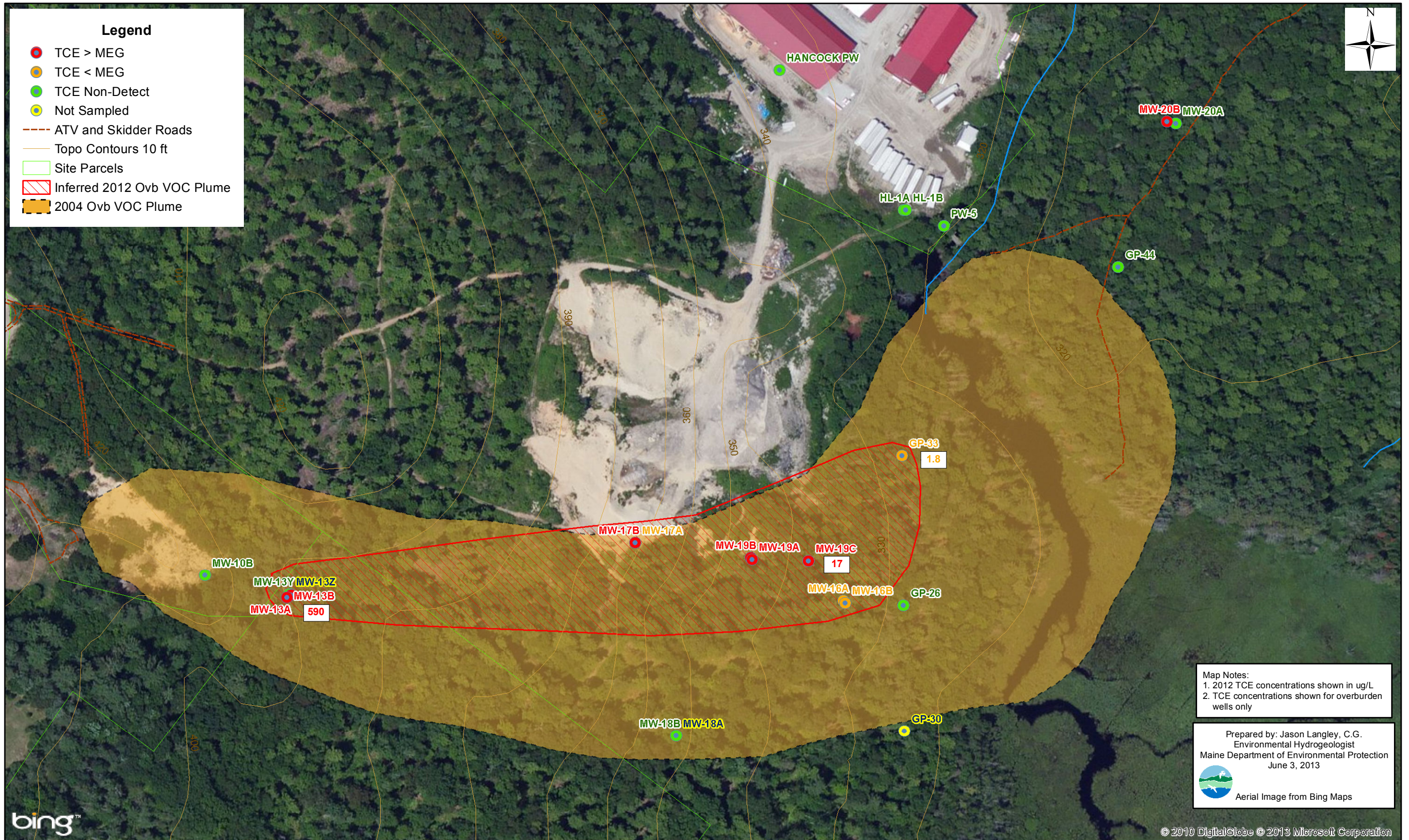
Figure 4B: Portland Bangor Waste Oil Casco Overburden VOC Plume 2004 vs. 2012
