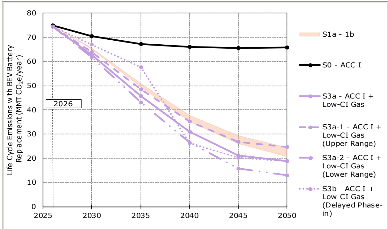
Figure 4-11: Life Cycle Emissions with BEV Battery Replacement for Alternative Scenarios Part 2
